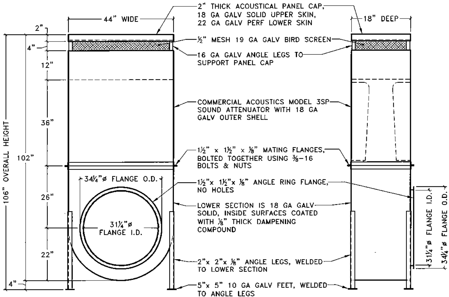
FRONT VIEW
